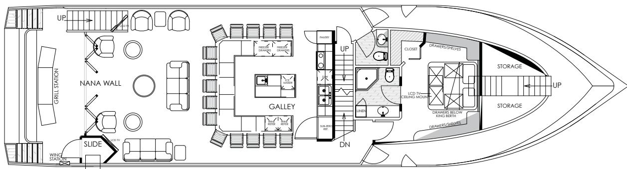
MAIN DECK ARRANGEMENT
