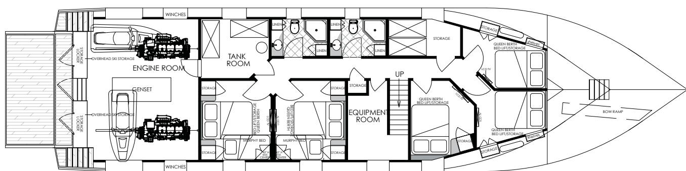
LOWER DECK ARRANGEMENT
